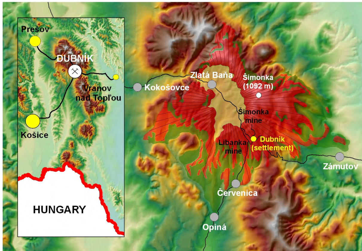
Maps showing position of the locality in the Slanské vrchy Mountain as well as the Zlatá Baňa stratovolcano (yellow – central zone, red – transitional zone, green – peripheral zone). Compiled by the Peter Semrád.
