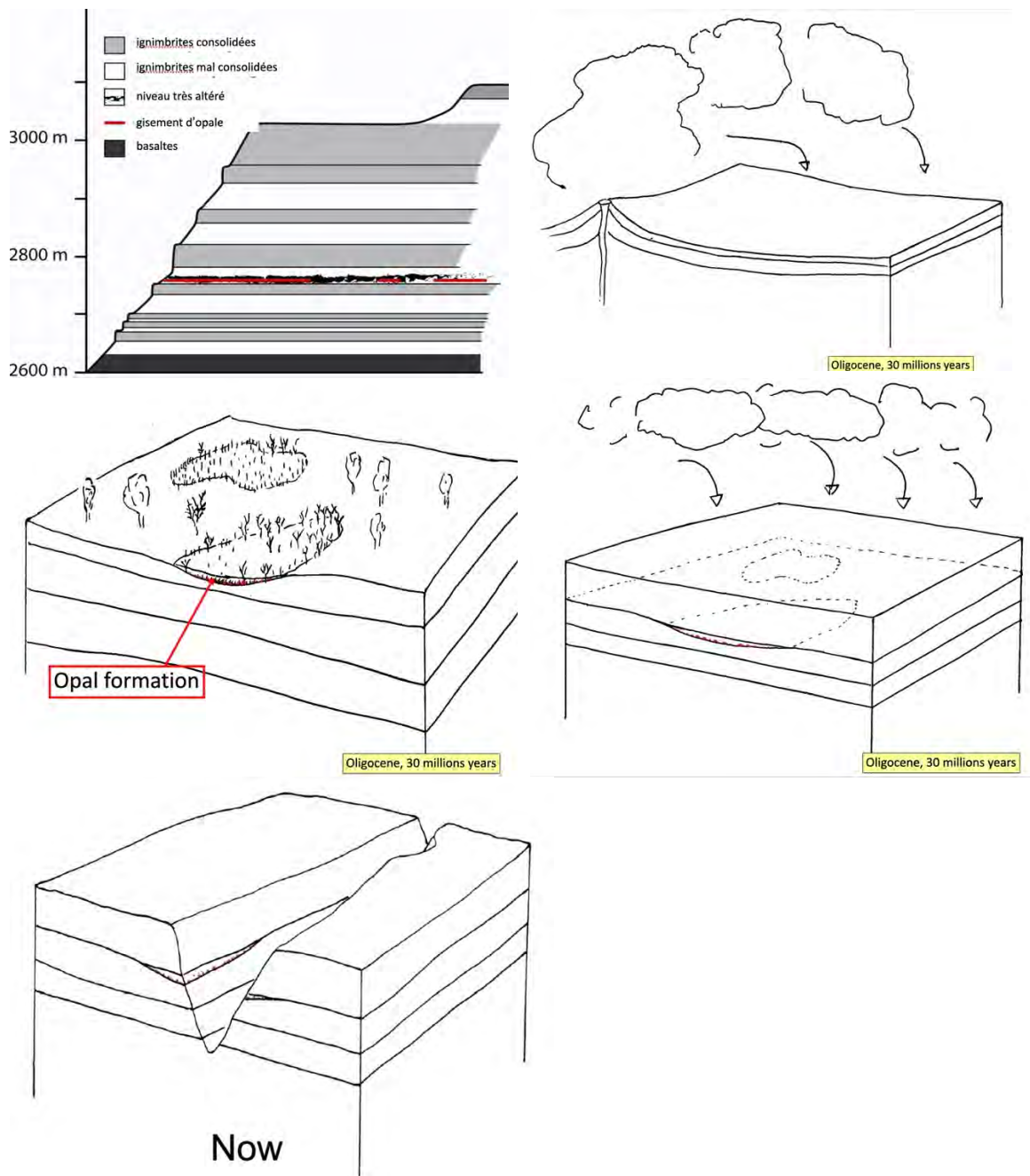
An illustration of the geological genesis of Ethiopian opal. Drawings by Benjamin Rondeau, see also (Chauvire 2017).
