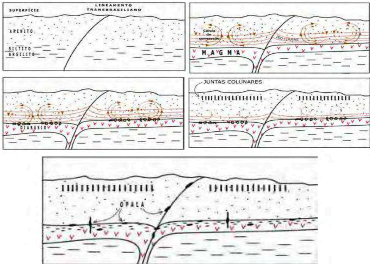
Schematic representation of the sedimentary rocks found in Pedro II, with sandstones at the top, siltstones and claystones at the base. Magma intrusion at the base of the sandstone, heating the fluids. Development of hydrothermal fluid convection cells. Hydraulic fracturing at the contact of the sedimentary rocks with the diabase sill. Intensifying hydrothermal alteration. Cooling of the hydrothermal system with the precipitation of opal in the fractures. (images: (Gomes 2022).
